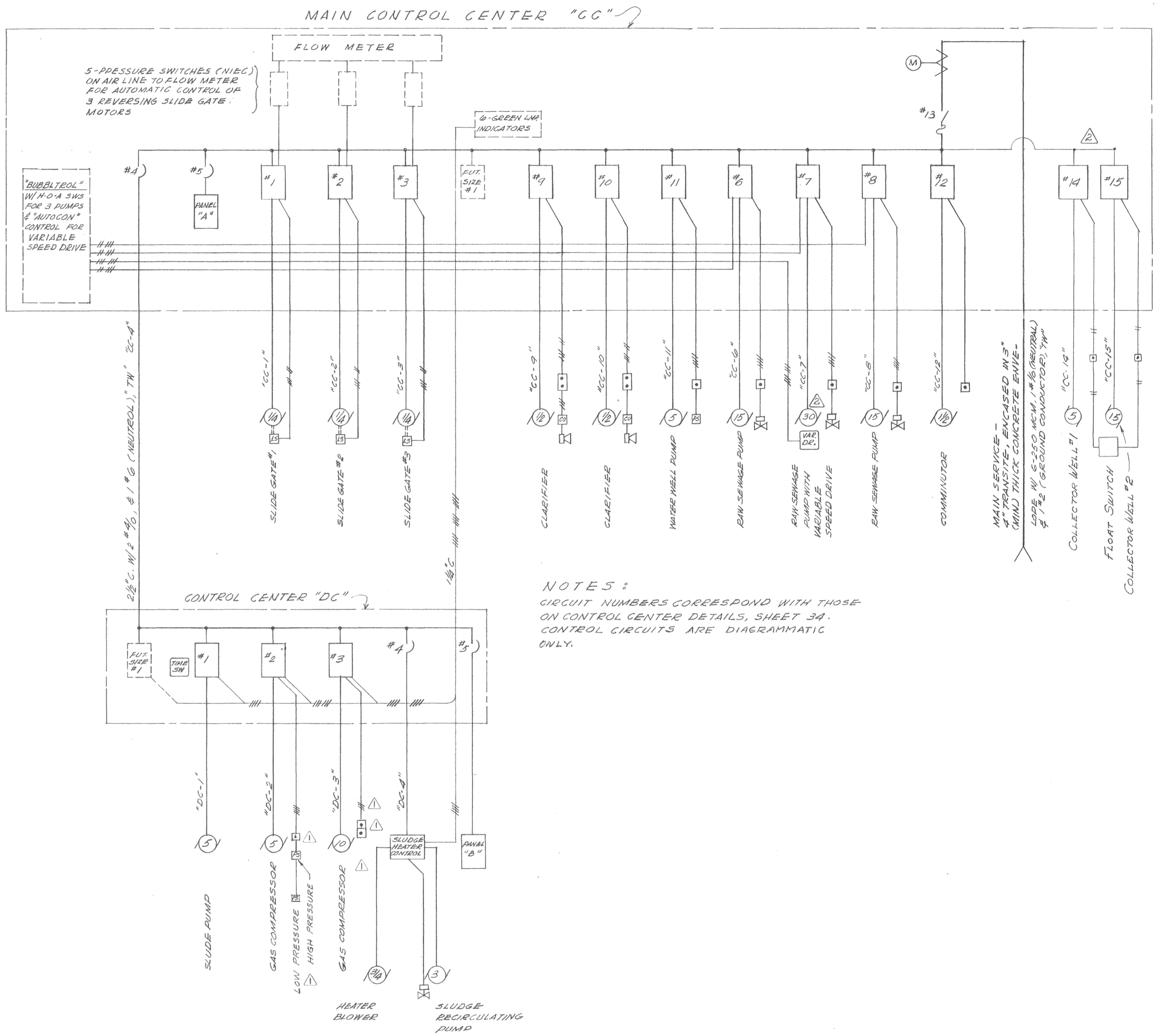
ONE LINE DIAGRAM AS BUILT NO SCALE
