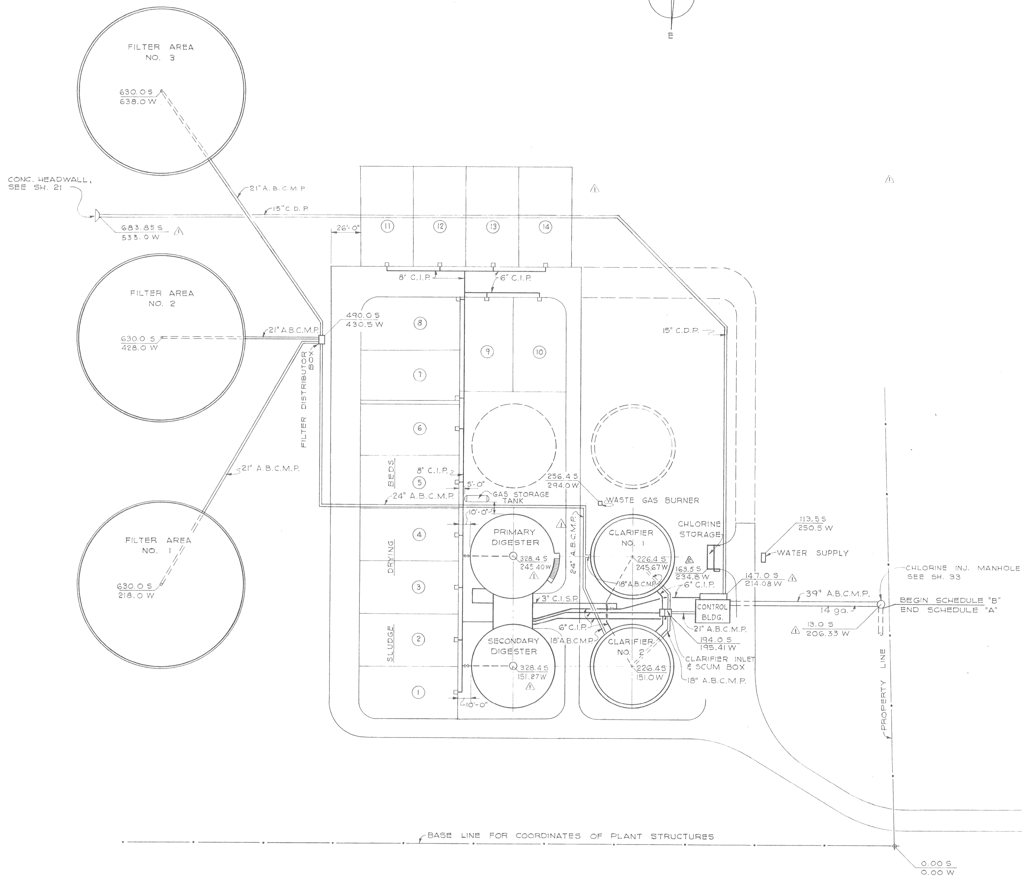
PLANT LAYOUT Scale: 1" = 40'
