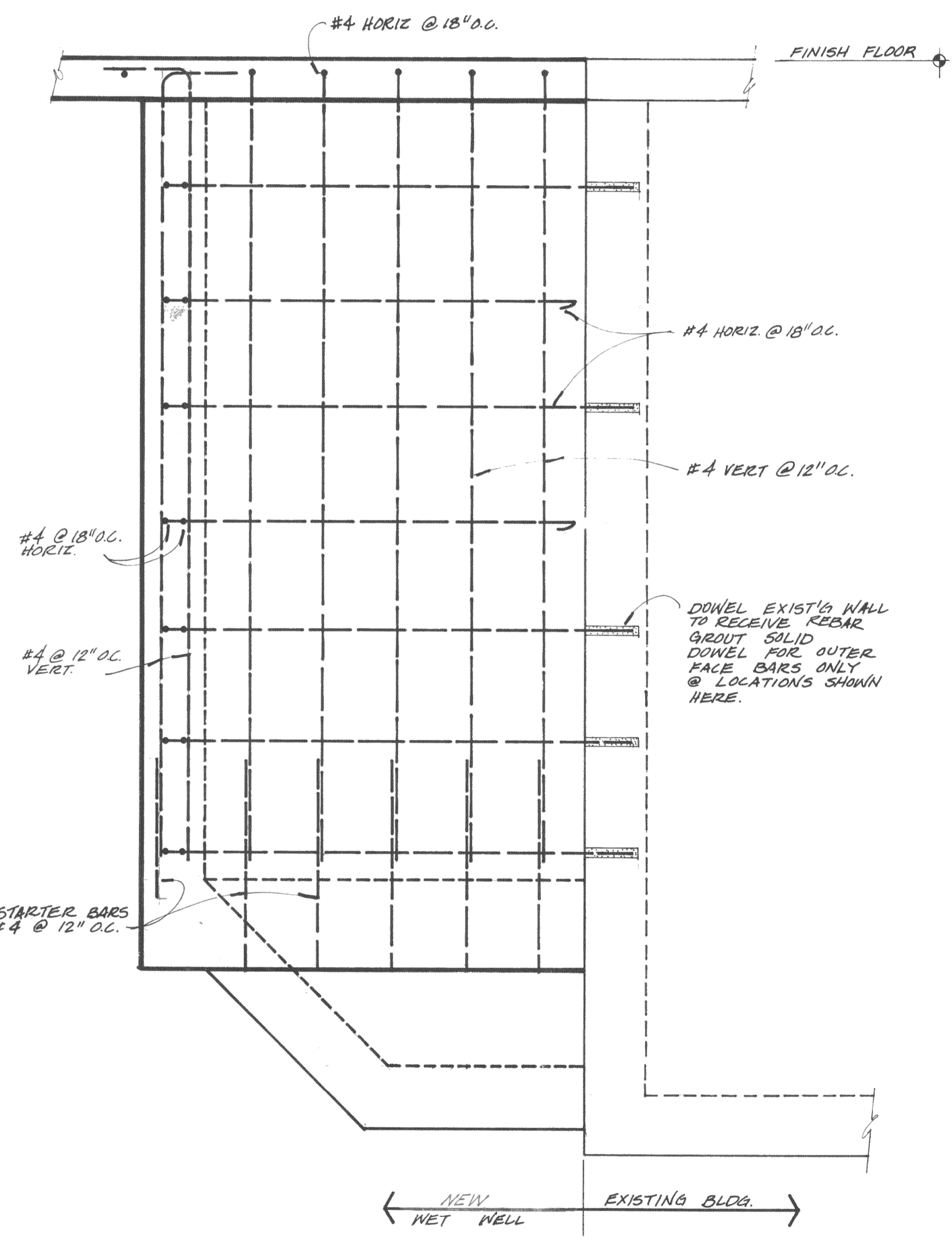
B REINFORCEMENT LAYOUT - END WALLS OF NEW WET WELL. 3/4" = 1'-0"
