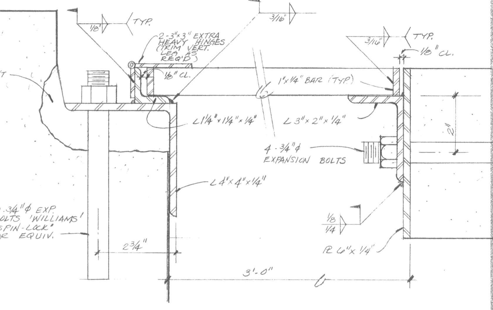
(K) NEW DRY-PIT ACCESS HATCH HALF-SIZE
