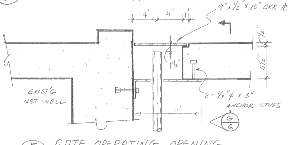
(F) GATE OPERATING OPENING 1 1/2" = 1'-0"
