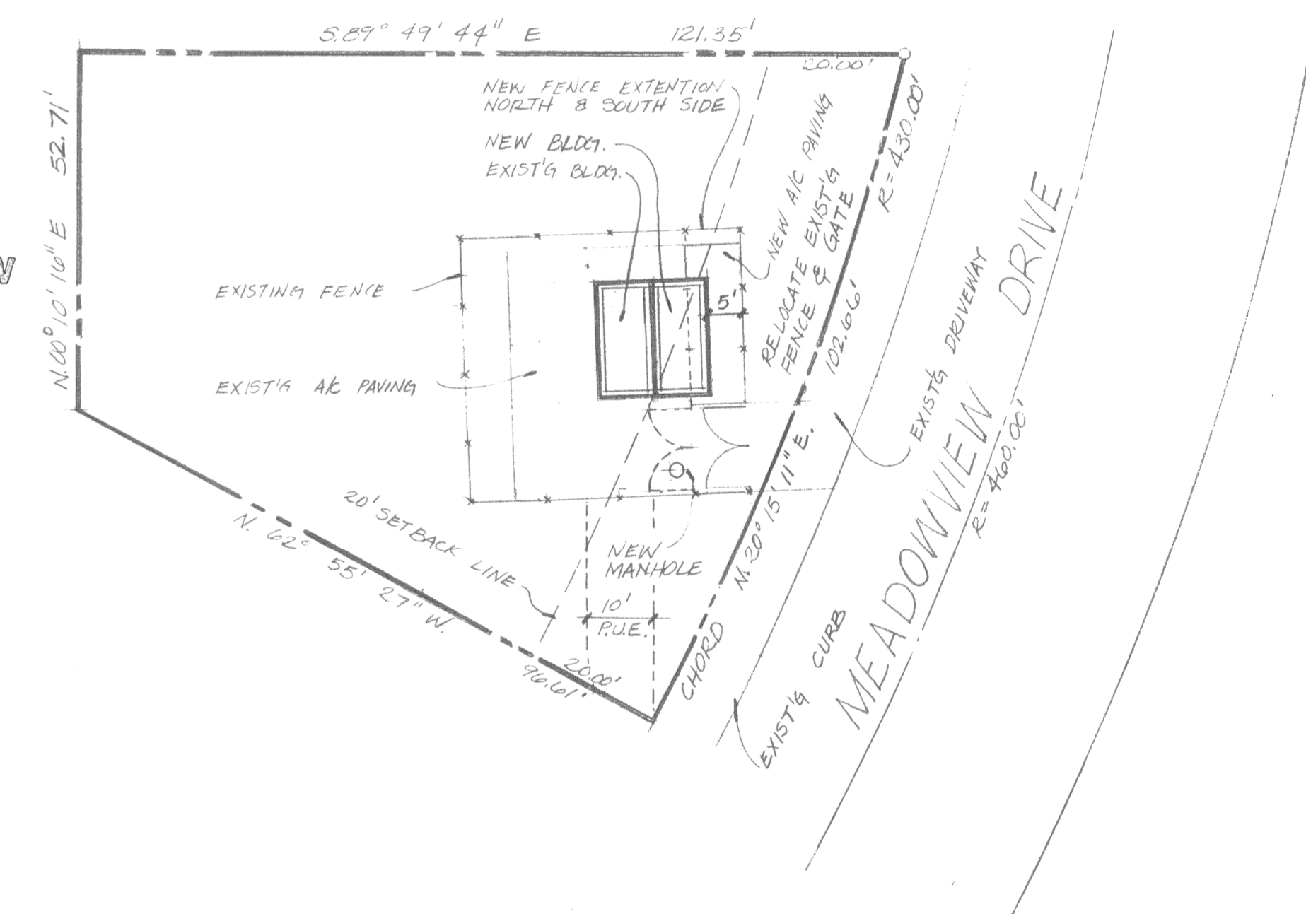
(B) SITE PLAN 1" = 20'-0"
