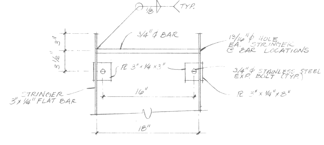
(B) LADDER DETAIL 1/2" = 1'-0"
