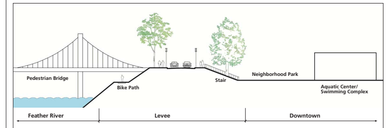
SECTION AT NEIGHBORHOOD PARK AND PEDESTRIAN BRIDGE
