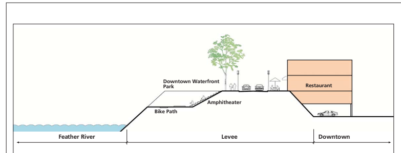
SECTION AT DOWNTOWN WATERFRONT PARK
