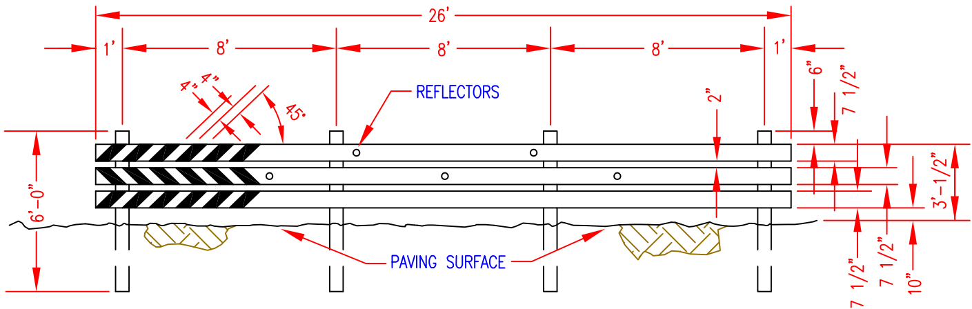
FRONT VIEW
