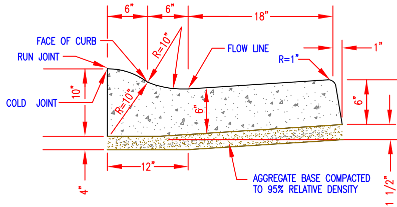
ROLLED CURB AND GUTTER
