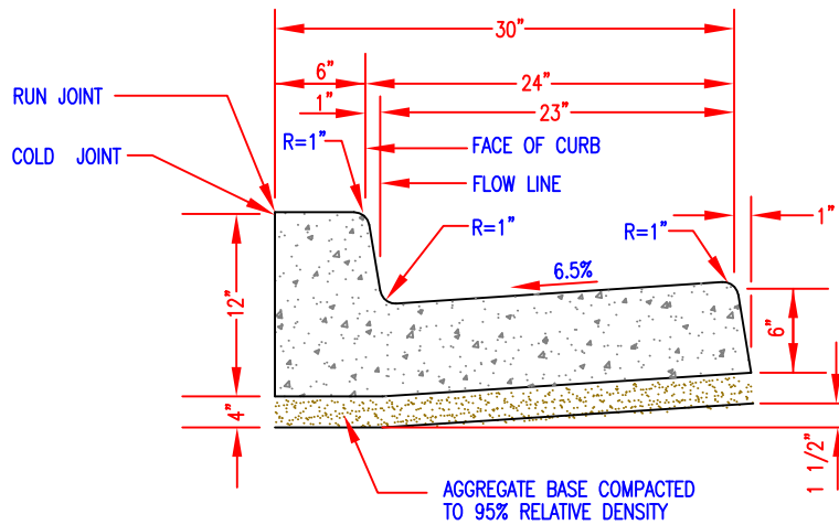
VERTICAL CURB AND GUTTER
