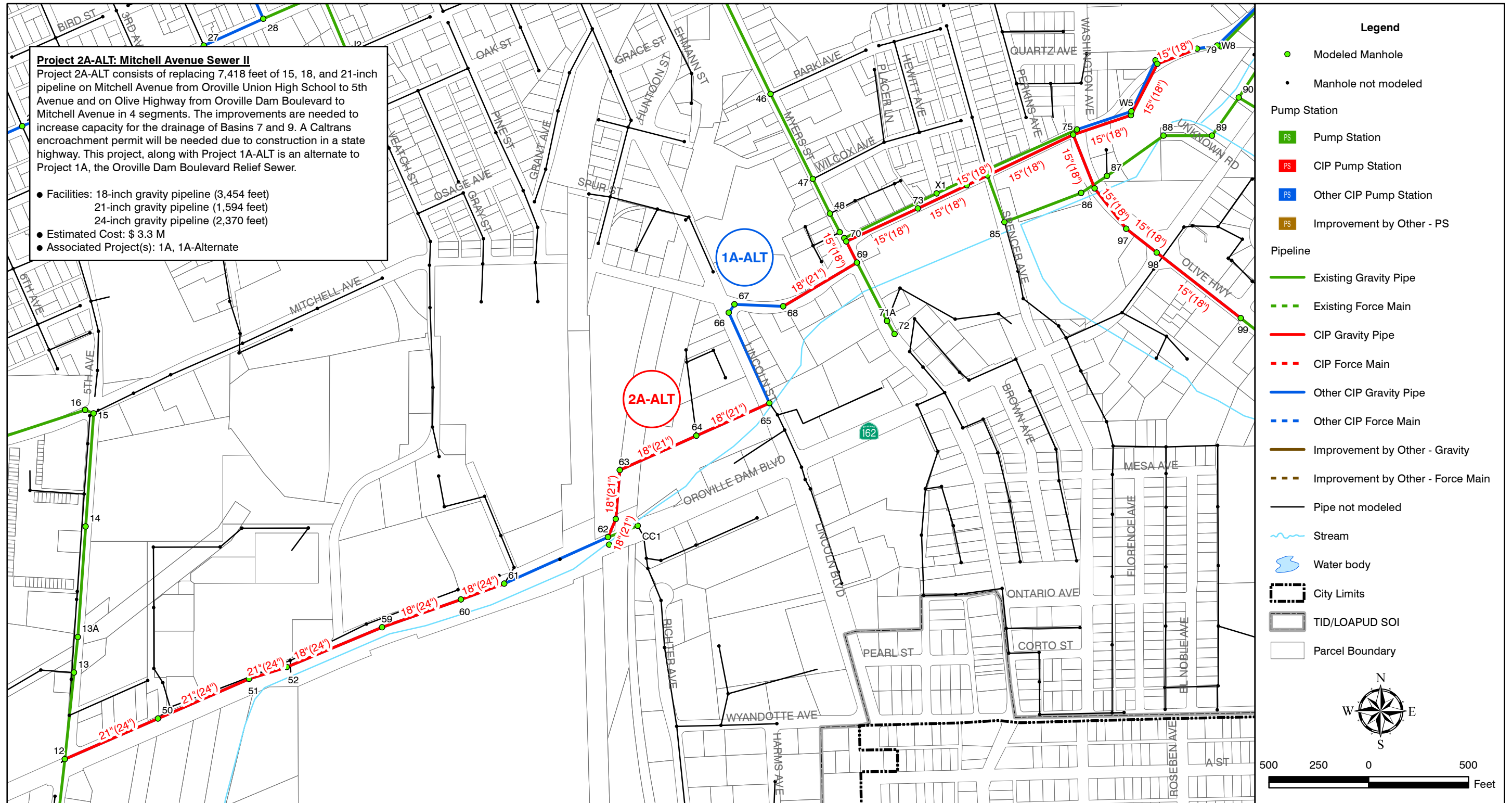
Figure 7.38 PROJECT 2A-ALTERNATE SANITARY SEWER MASTER PLAN CITY OF OROVILLE
