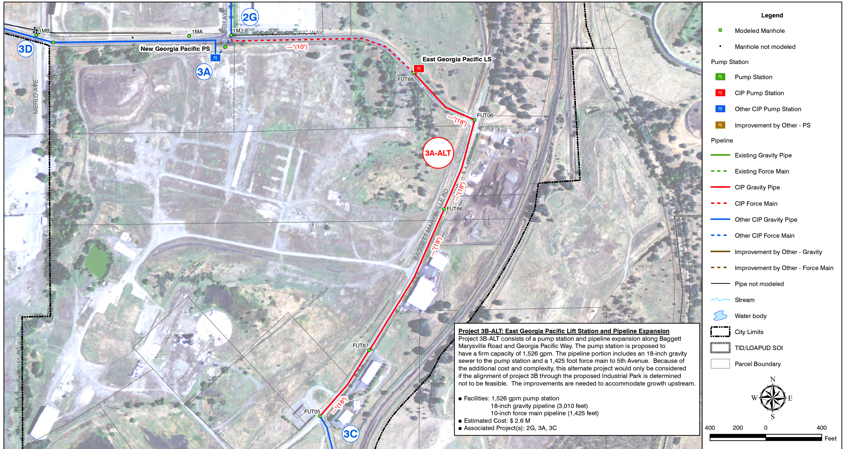
Figure 7.39 PROJECT 3B-ALTERNATE SANITARY SEWER MASTER PLAN CITY OF OROVILLE
