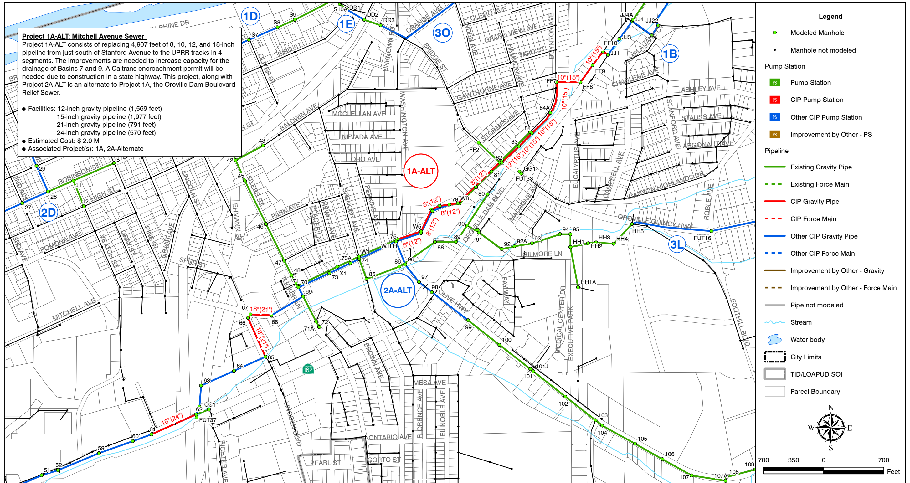
Figure 7.37 PROJECT 1A-ALTERNATE SANITARY SEWER MASTER PLAN CITY OF OROVILLE
