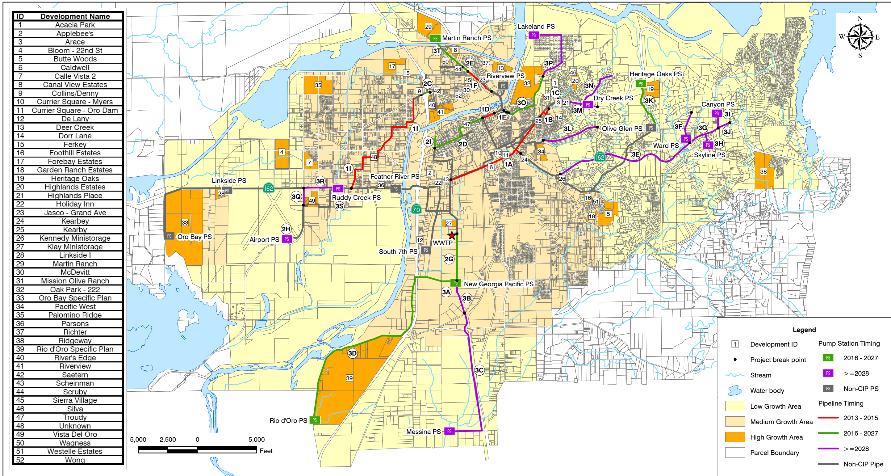
Figure 7.36 CIP PHASING SANITARY SEWER MASTER PLAN CITY OF OROVILLE
