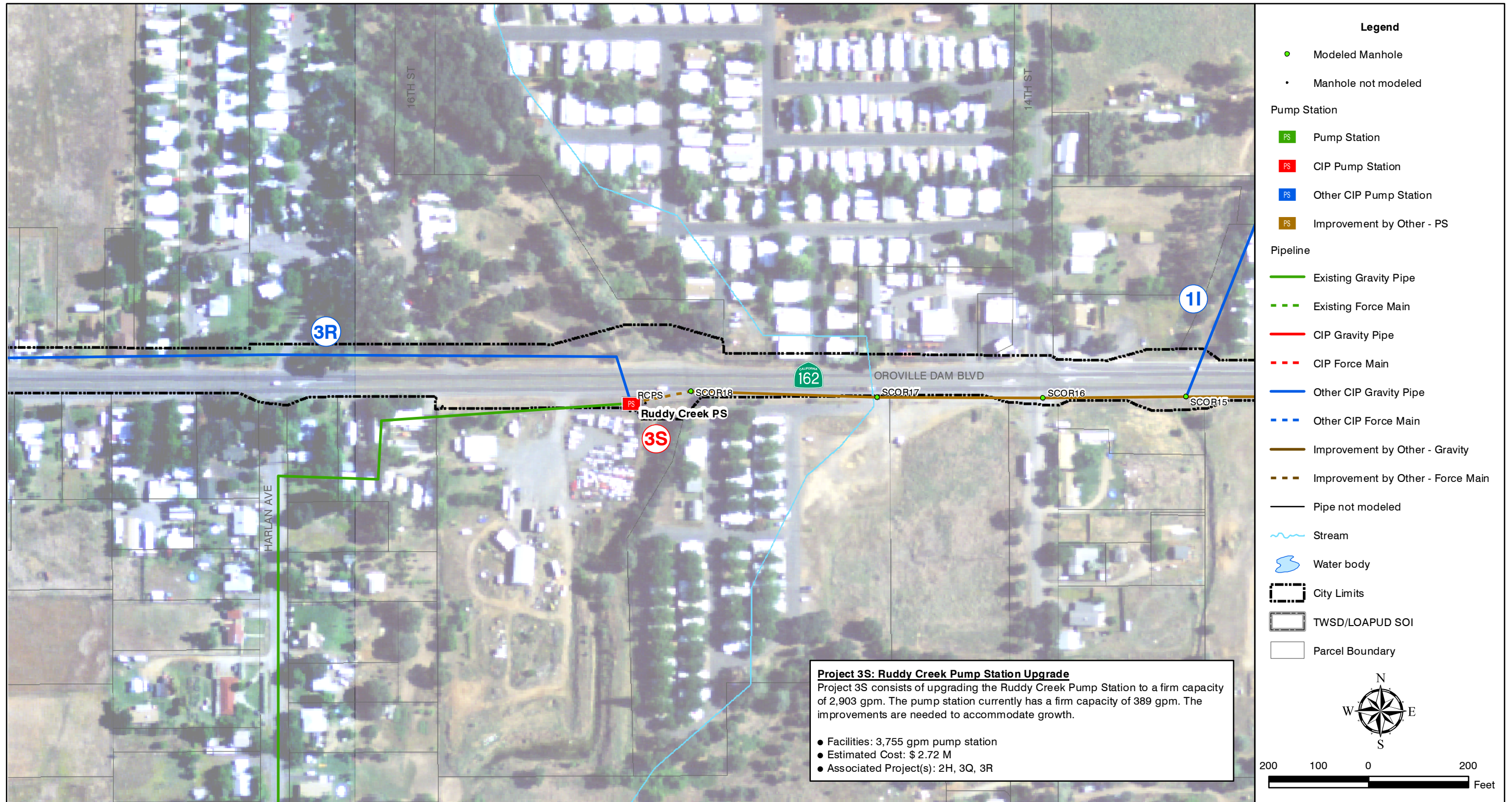
Figure 7.33 PROJECT 3S SANITARY SEWER MASTER PLAN CITY OF OROVILLE
