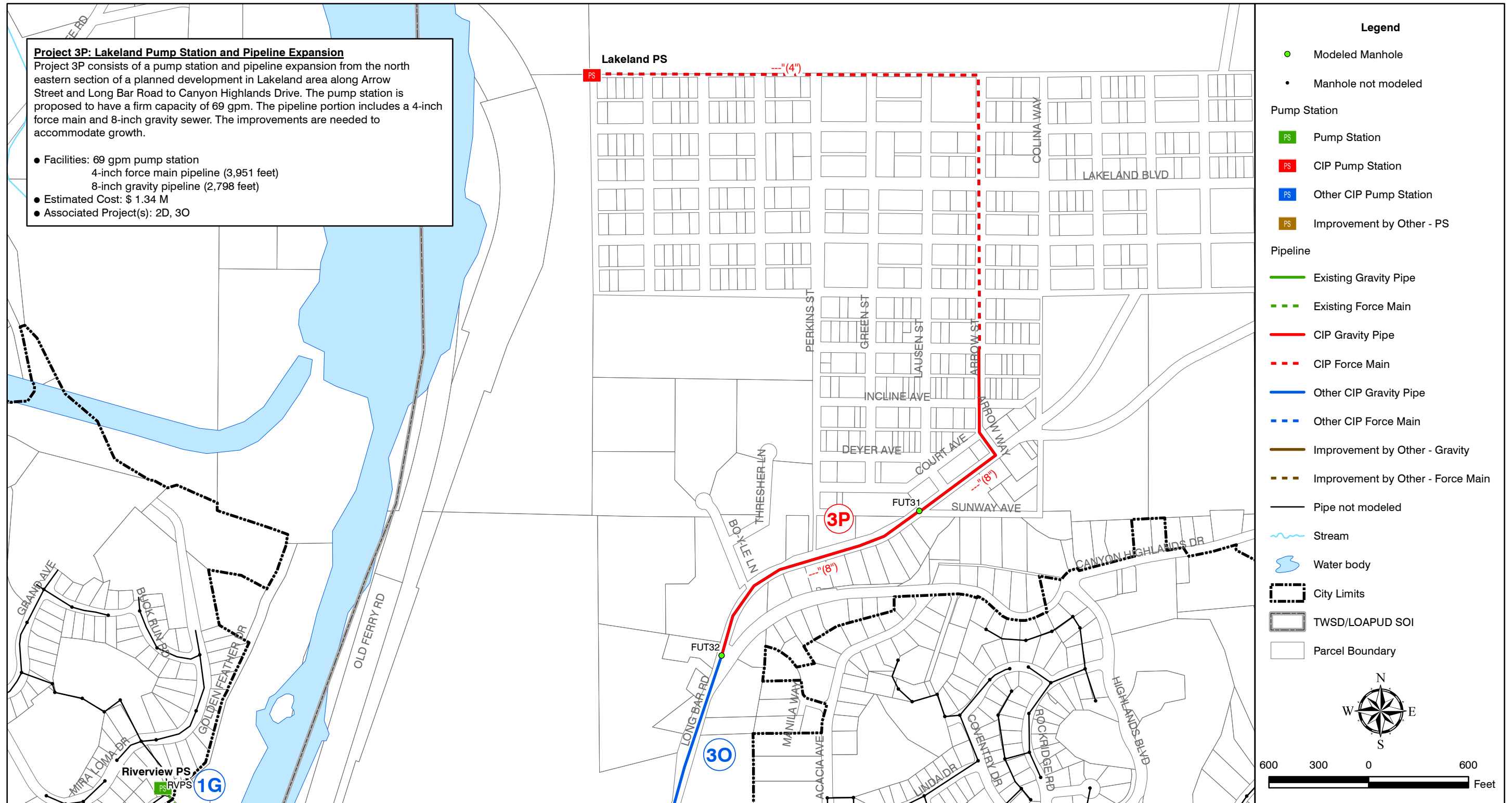
Figure 7.30 PROJECT 3P SANITARY SEWER MASTER PLAN CITY OF OROVILLE
