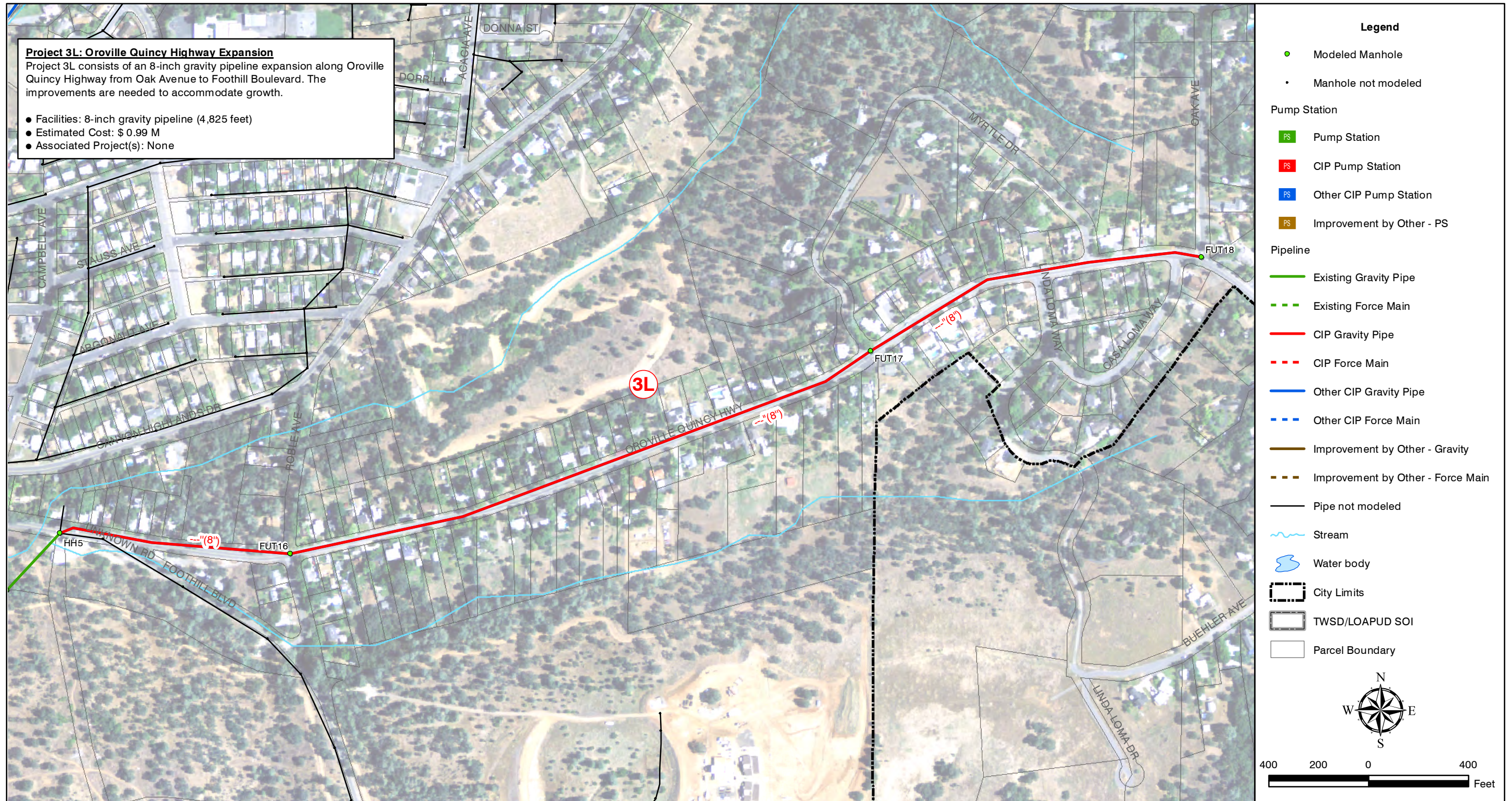
Figure 7.26 PROJECT 3L SANITARY SEWER MASTER PLAN CITY OF OROVILLE
