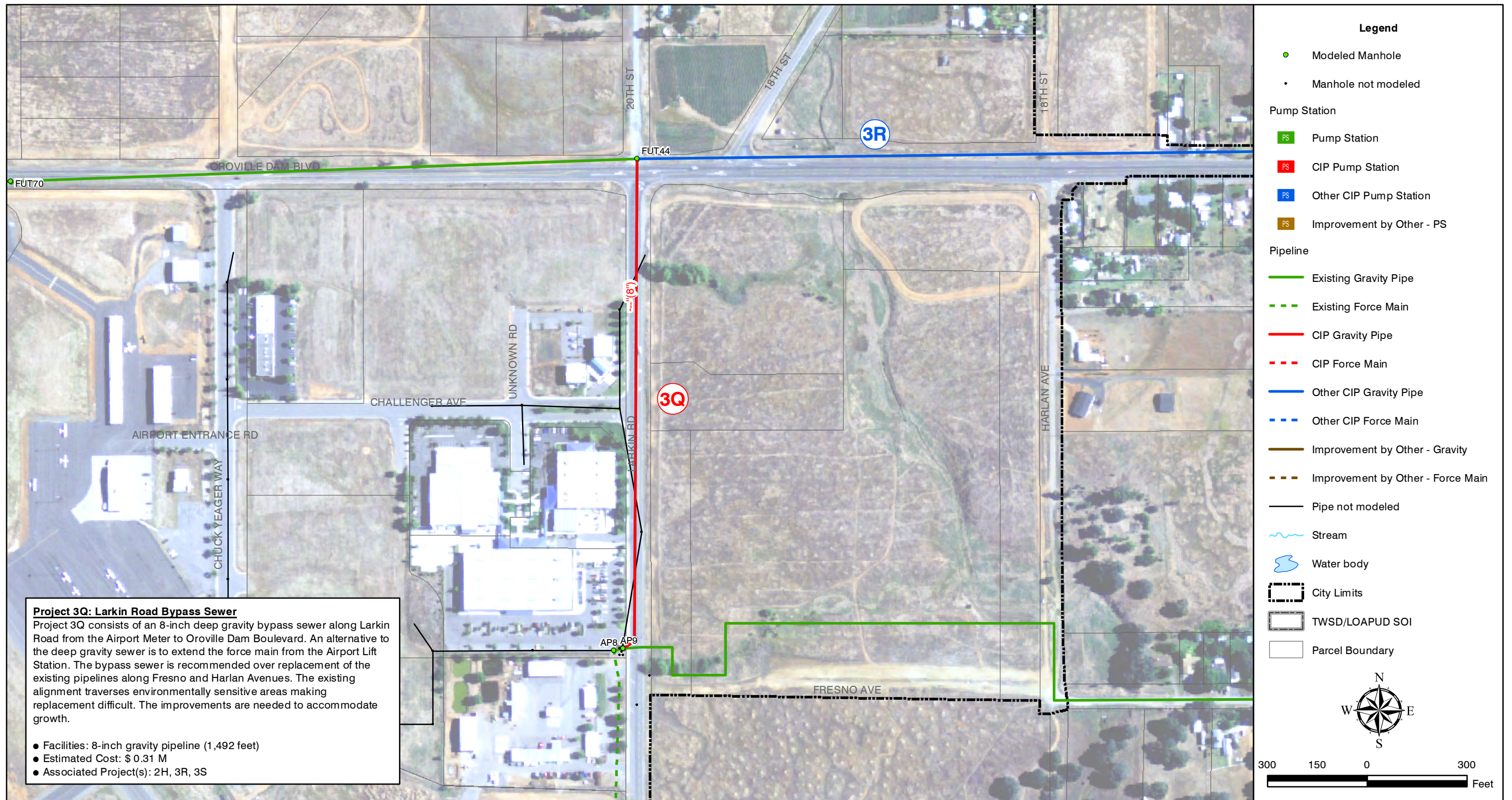
Figure 7.31 PROJECT 3Q SANITARY SEWER MASTER PLAN CITY OF OROVILLE
