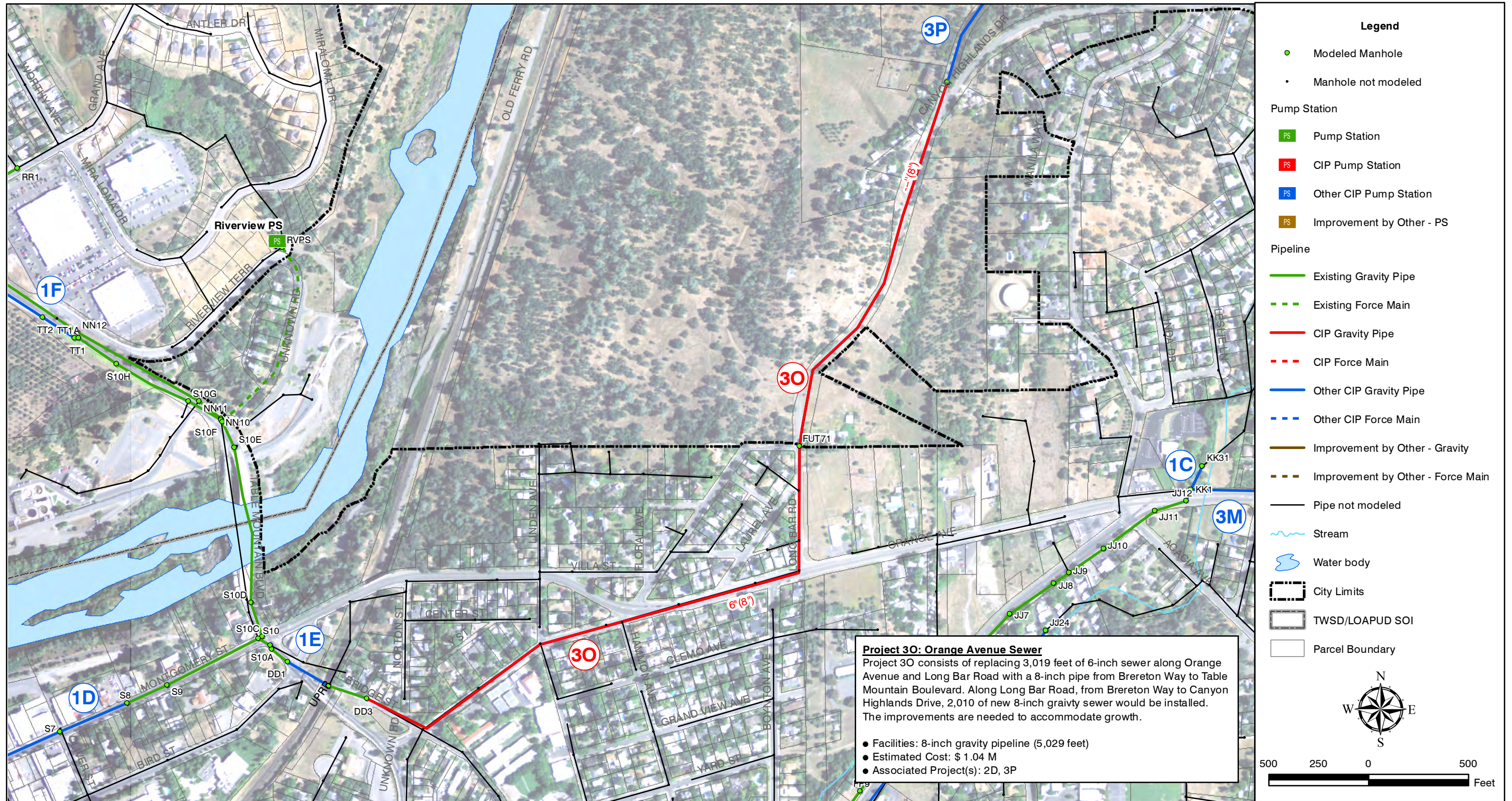
Figure 7.29 PROJECT 30 SANITARY SEWER MASTER PLAN CITY OF OROVILLE
