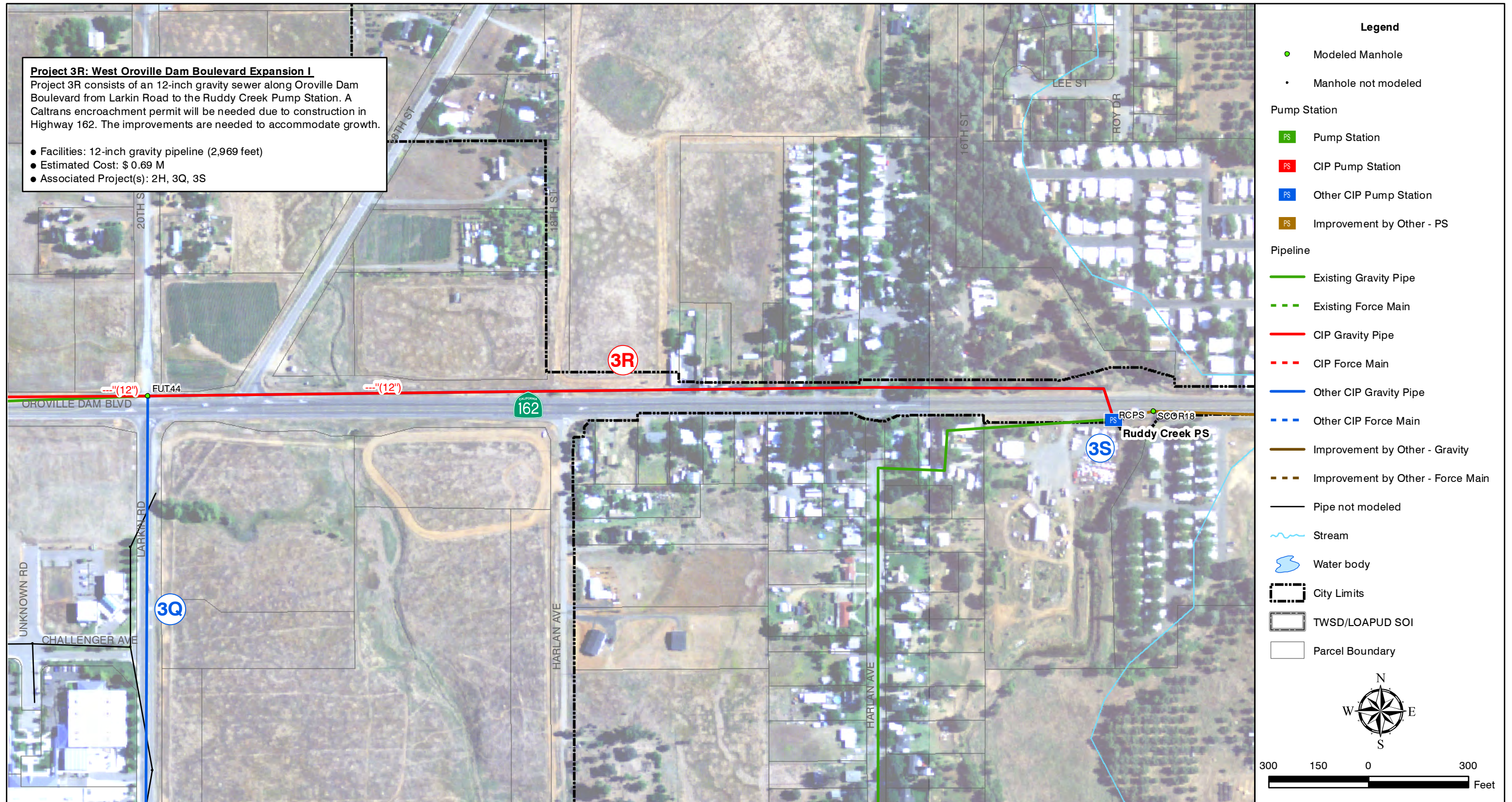
Figure 7.32 PROJECT 3R SANITARY SEWER MASTER PLAN CITY OF OROVILLE
