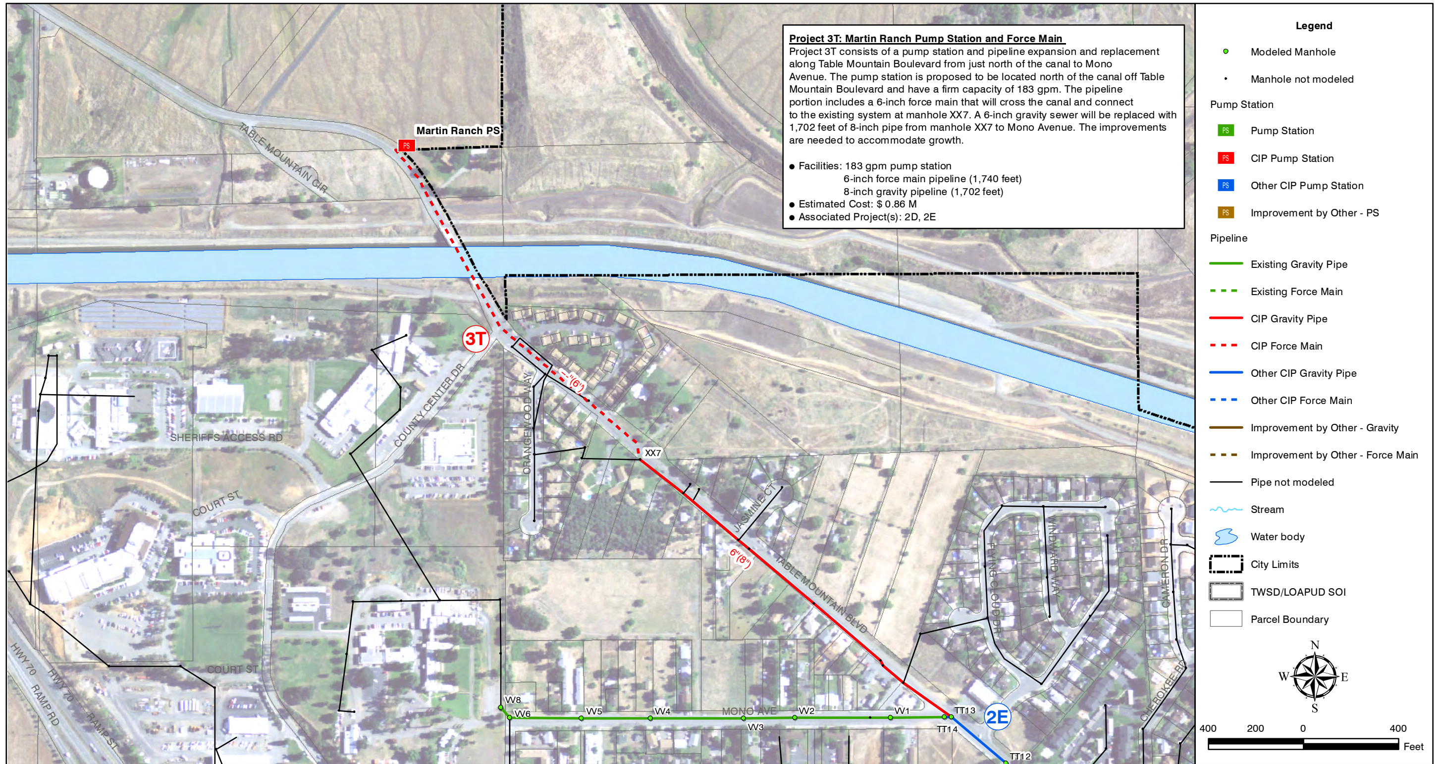
Figure 7.34 PROJECT 3T SANITARY SEWER MASTER PLAN CITY OF OROVILLE
